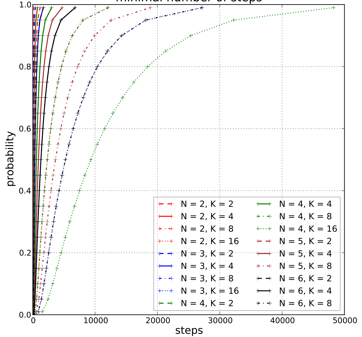
minimal number of steps
