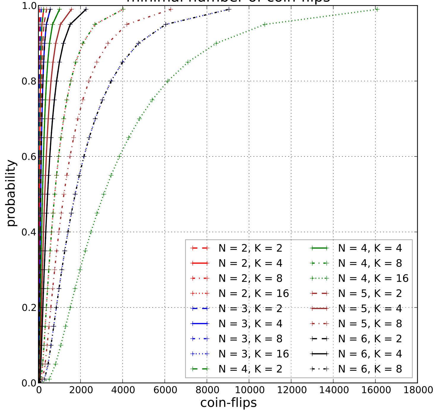
minimal number of coin-flips
